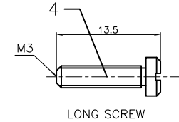
LONG SCREW
