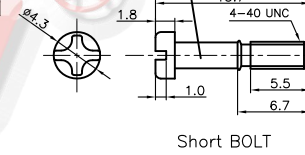
Short BOLT
