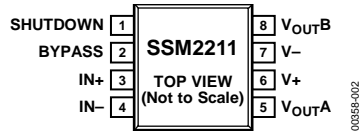
Figure 2. 8-Lead SOIC_N Pin Configuration (R-8)
