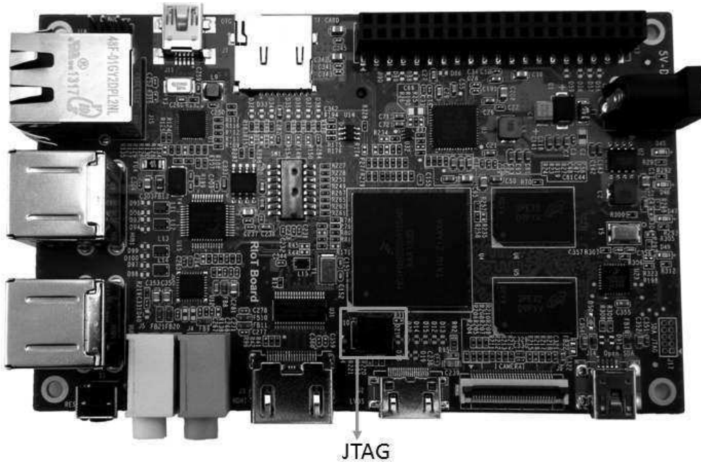
Figure 2-11 JTAG Interface
