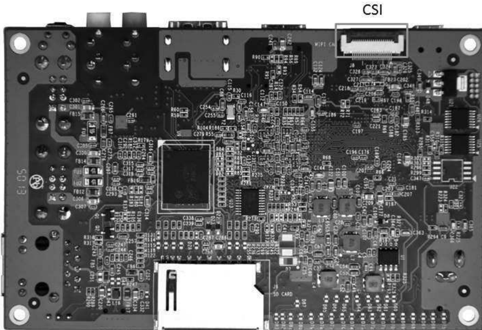
Figure 2-9 CSI Interface
