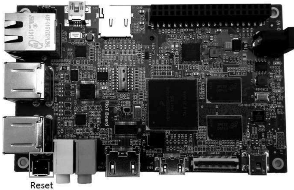
Figure 2-19 Reset Switch
