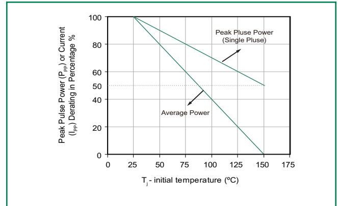
Figure 2 - Peak Pulse Power or Current Derating Curve vs Initial Junction Temperature
