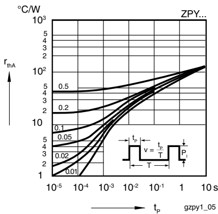
Figure 2. Pulse Thermal Resistance vs. Pulse Duration
