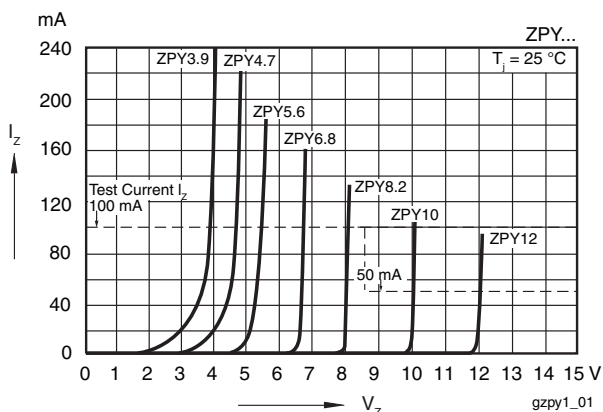
Figure 7. Breakdown Characteristics
