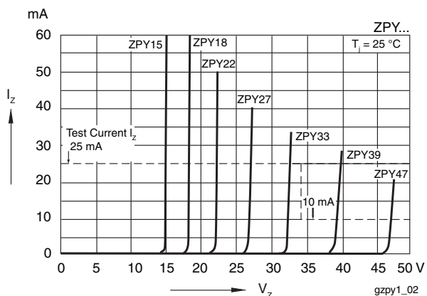
Figure 8. Breakdown Characteristics
