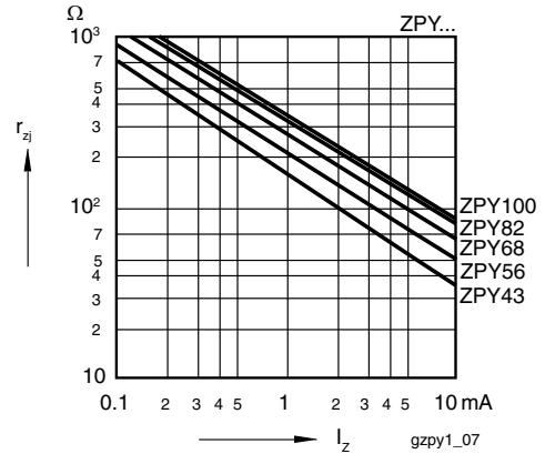
Figure 4. Dynamic Resistance vs. Zener Current
