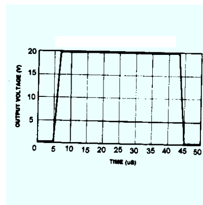
Figure 6. Slew Rate
