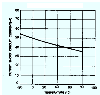
Figure 5. Output Circuit Current vs Temperature
