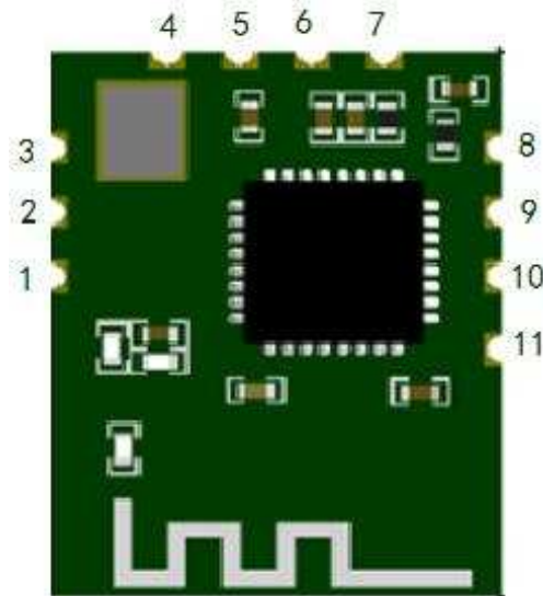
Fig. 2. Module Pins Distribution Diagram (Top View)
