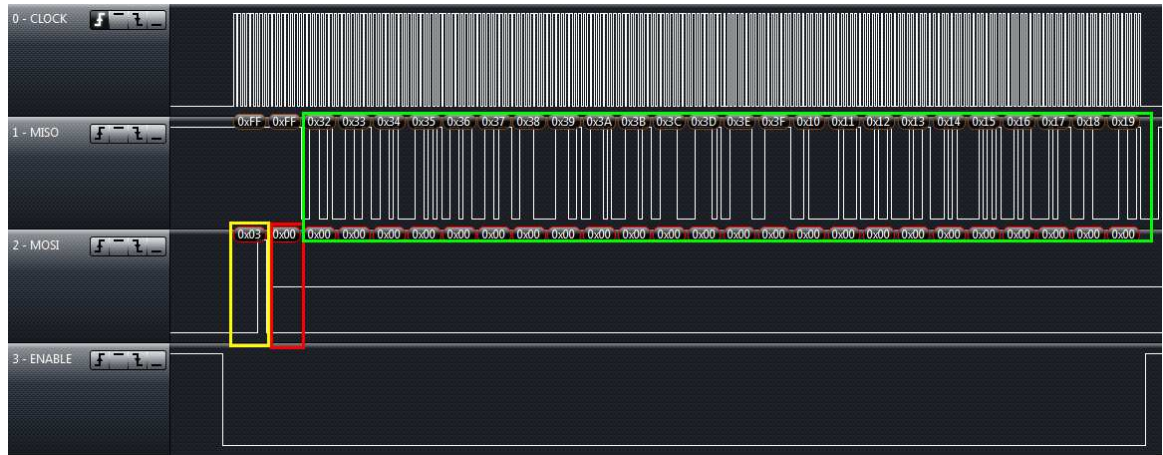
Figure 4-6. Waveform Graph 2
