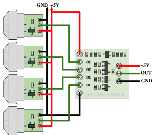
Example wiring with 4pcs PIRMINI
