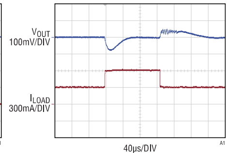
Load Transient, V OUT = 5V
