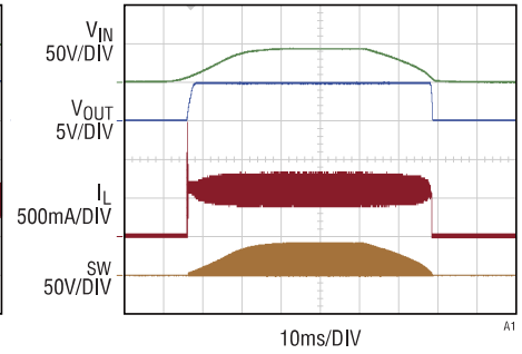
Power Up and Power Down EN = V IN
