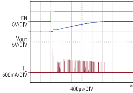
Start-Up Waveforms NO LOAD
