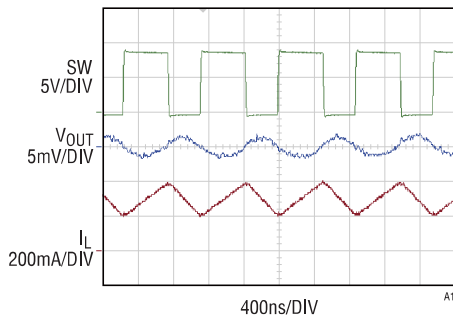
Switching Waveforms, PWM Mode
