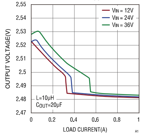
Load Regulation, V_{OUT} = 2.5\text{V}
