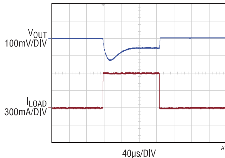
Load Transient, V OUT = 5V
