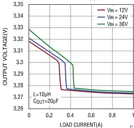
Load Regulation, V_{OUT} = 3.3\text{V}
