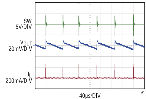
Switching Waveforms, Pulse Skip Mode
