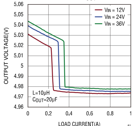
Load Regulation, V_{OUT} = 5\text{V}
