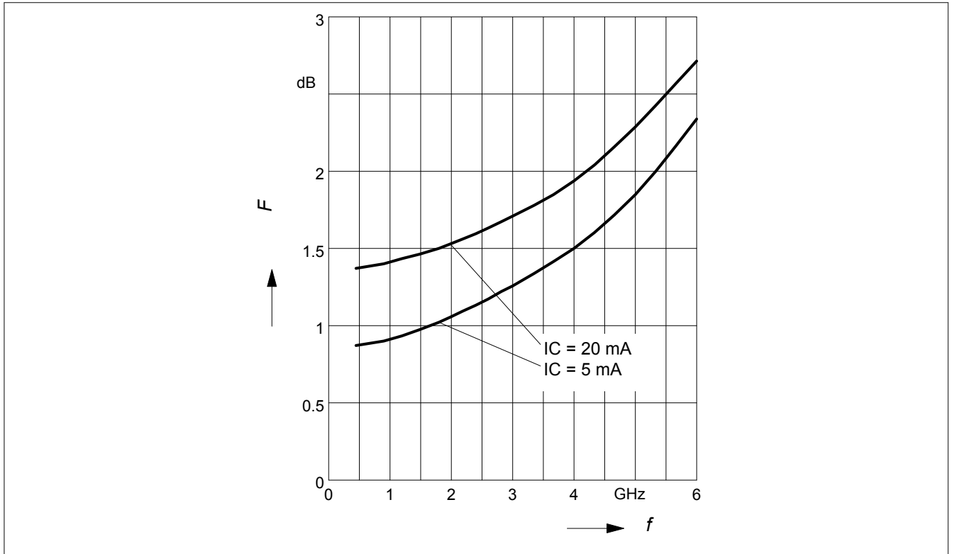
Figure 17 Noise figure NF_{\min} = f(f) , V_{CE} = 2\text{ V} , Z_S = Z_{S,opt} , I_C = 5 / 20\text{ mA}
