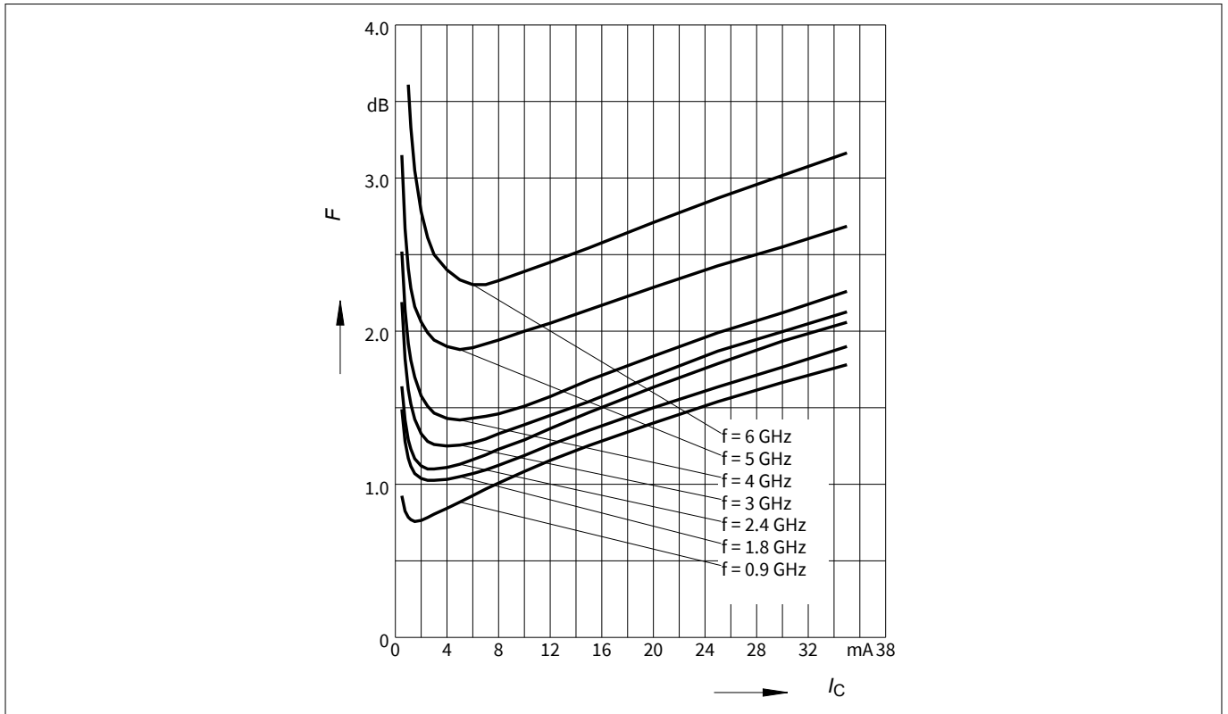
Figure 18 Noise figure NF_{\min} = f(I_C) , V_{CE} = 2\text{ V} , Z_S = Z_{S,opt} , f = \text{parameter in GHz}
