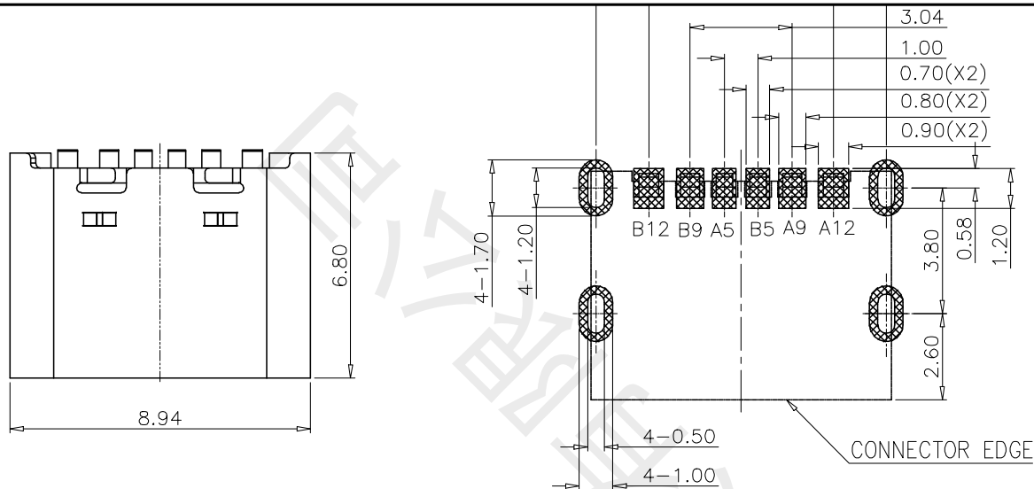
RECOMMENDED PCB LAYOUT(TOP VIEW) THICKNESS 1.6±0.10MM;DEFAULT TOLERANCE:±0.05
