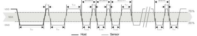
Figure 8 AM2120 Single bus communication timing
