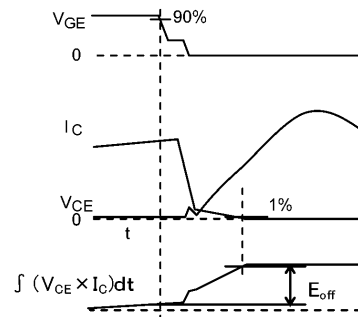
Fig. 6.2.4 Timing Chart of Switching Loss
