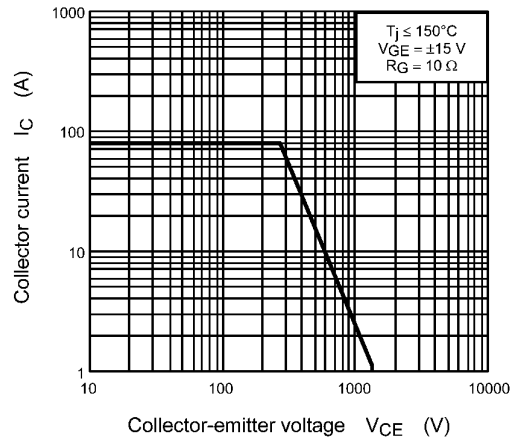
Fig. 8.10 Reverse Bias SOA (Guaranteed Maximum)
