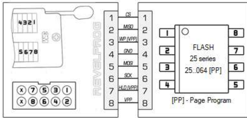
Straight connection „1 to 1“ for FLASH SPI
