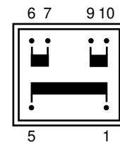
Primary winding
