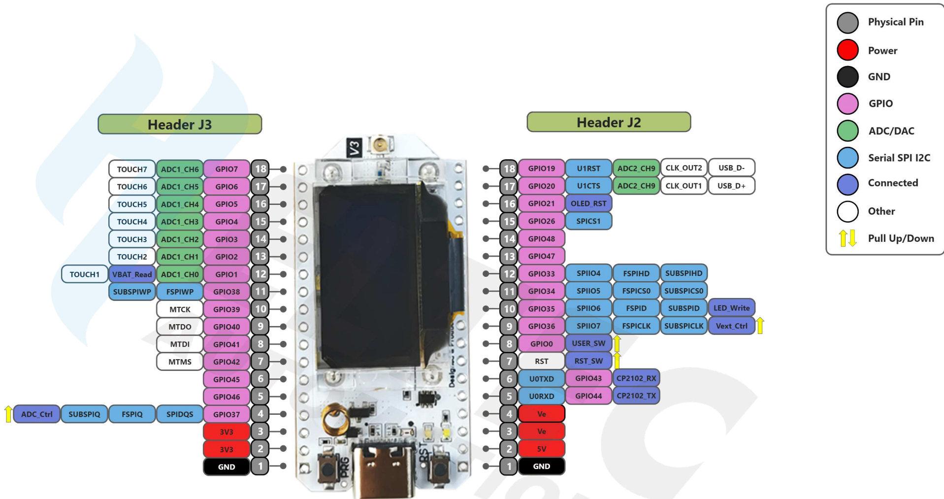
HTIT-WB32LA(F)_V3 Pin map
