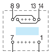
1 Secondary winding 8 9 13 14
