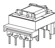
EF 16 reinforced insulation creepage distances: 6mm
