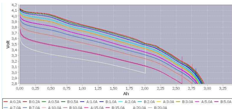
Discharge characteristics of the cell ICR18650-300PCM-R
