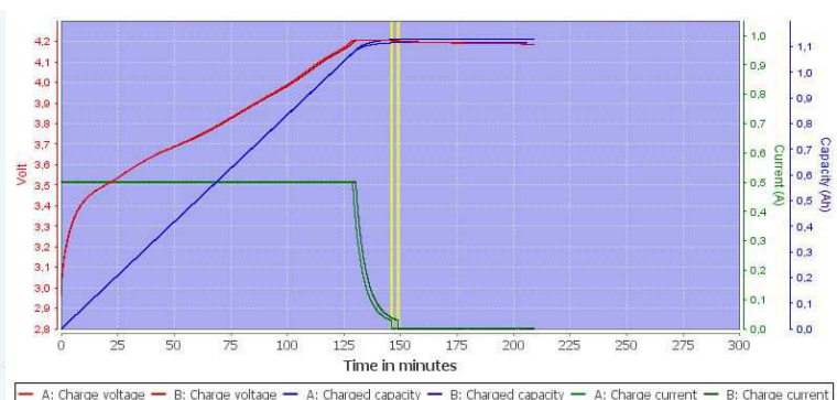
Characteristics of charging the cell ICR18650-300PCM-R
