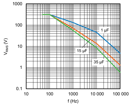
Maximum RMS voltage as function of frequency T_{amb} \leq 85\text{ }^{\circ}\text{C} ; U_r = 310\text{ V}_{AC}
