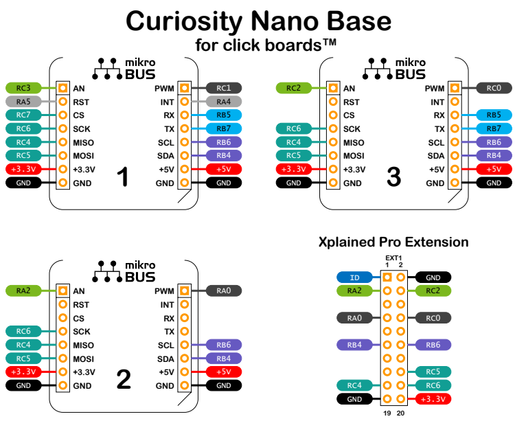
Figure 8-4. PIC18F16Q40 Curiosity Nano Pinout Mapping
