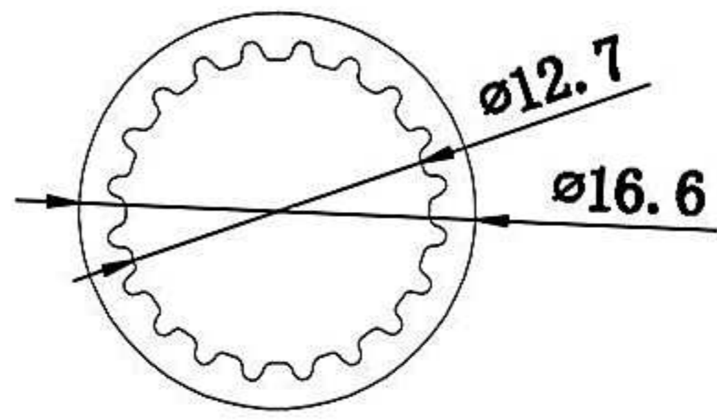
WASHER 1 PCS T=0.5
