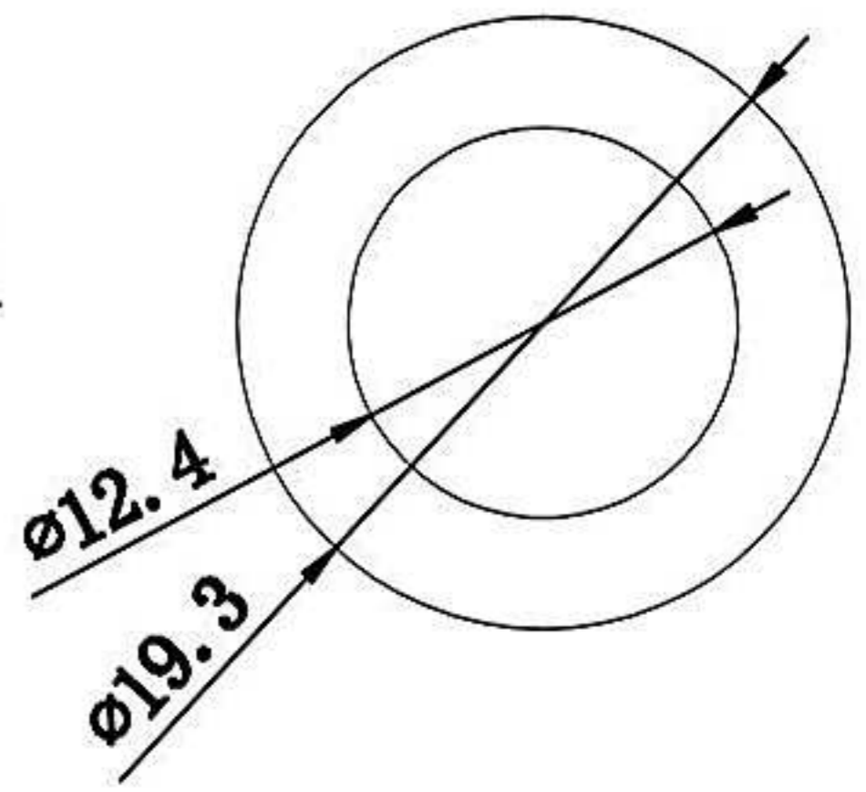
WASHER 1 PCS T=1.4
