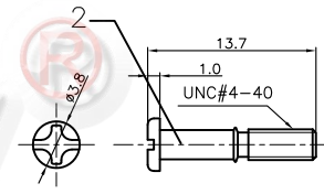
Short BOLT
