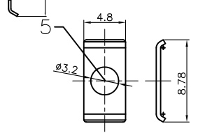
SMALL WASHER
